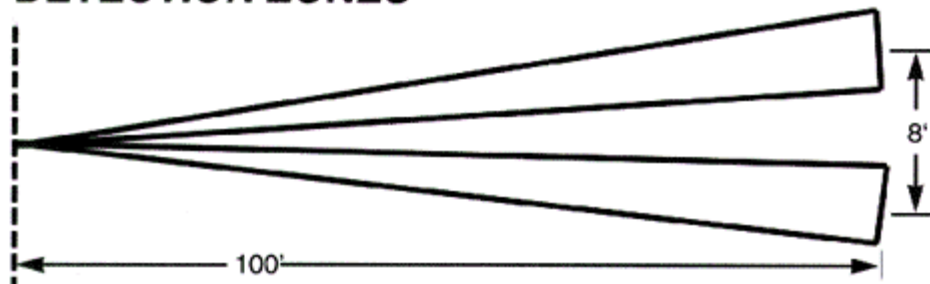
TOP VIEW - Intruder must cross A & B zones for trip
